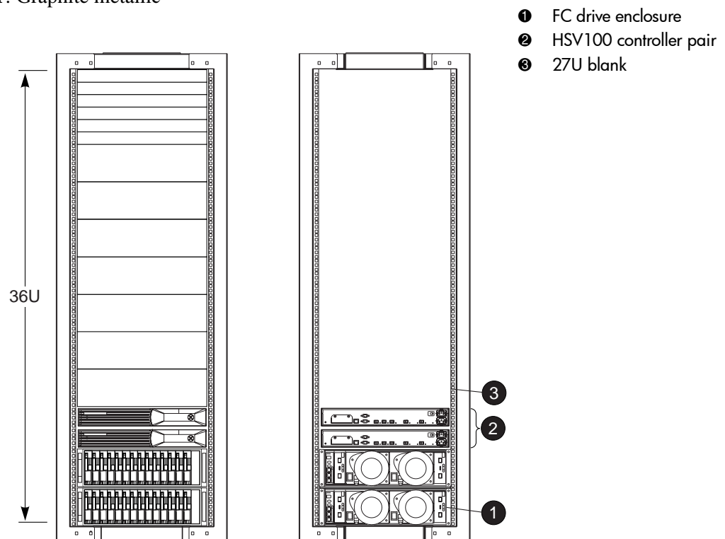
Figure 2: 36U rack -- front and rear views
