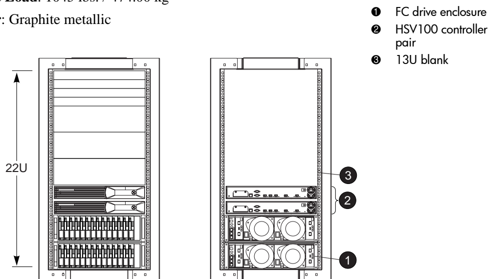
Figure 1: 22U rack -- front and rear views
